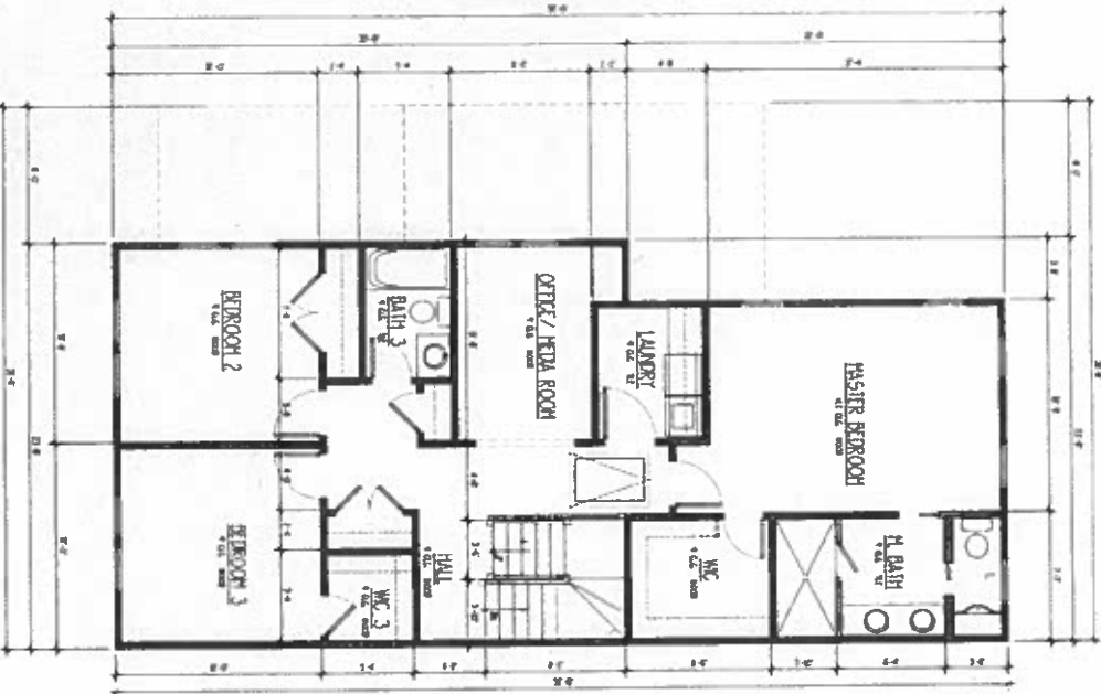
SECOND FLOOR PLAN 1092 sq. ft.
