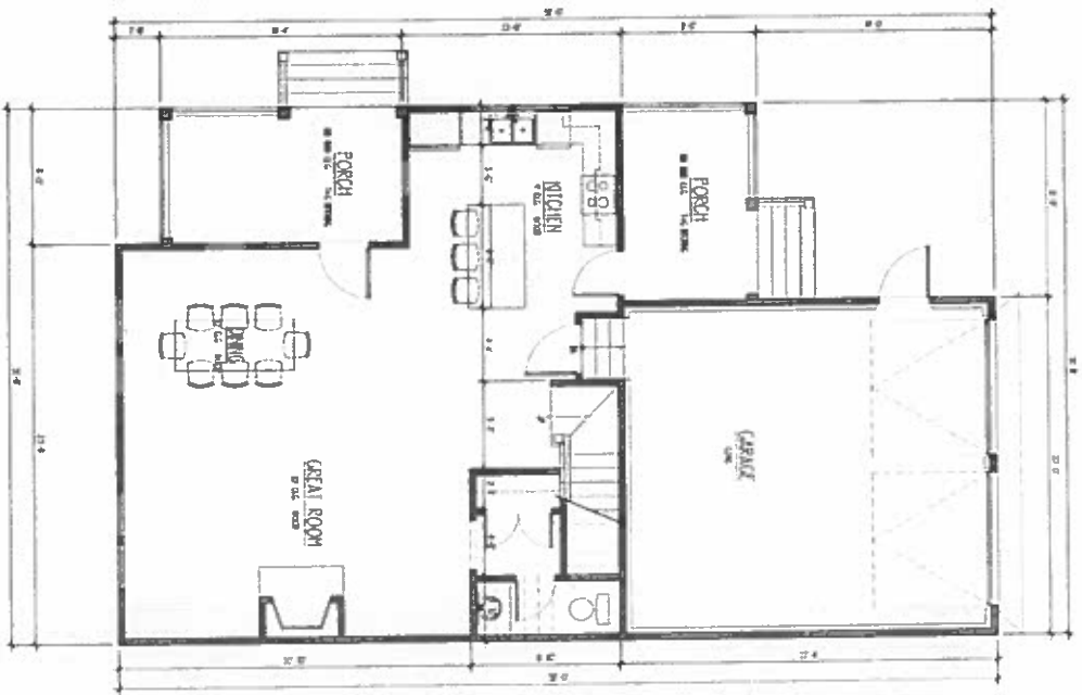
FIRST FLOOR PLAN 813 sq. ft.
